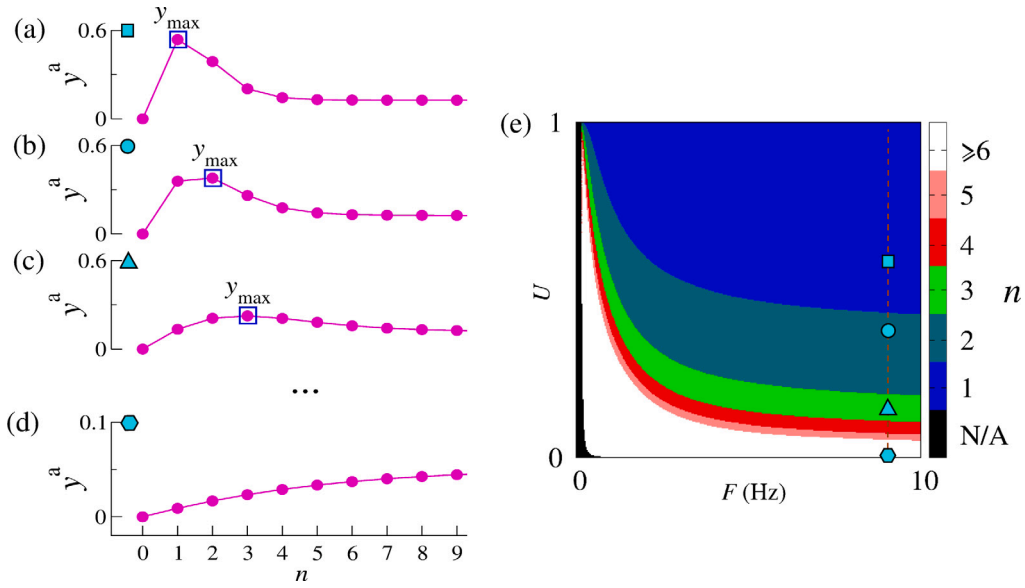
Fig. 4. y variable after the spike ( y^o ) for different values of the parameter of U identifying the maximal value ( y_{\max} ). In Fig. (a–d), we fix F = 9 Hz, (a) U = 0.6 , (b) U = 0.4 , (c) U = 0.15 and (d) U = 0.01 . Fig. (e) shows the number of iterations to find the maximal value of y from the rest state of the synapse. (For interpretation of the references to colour in this figure legend, the reader is referred to the web version of this article.)
