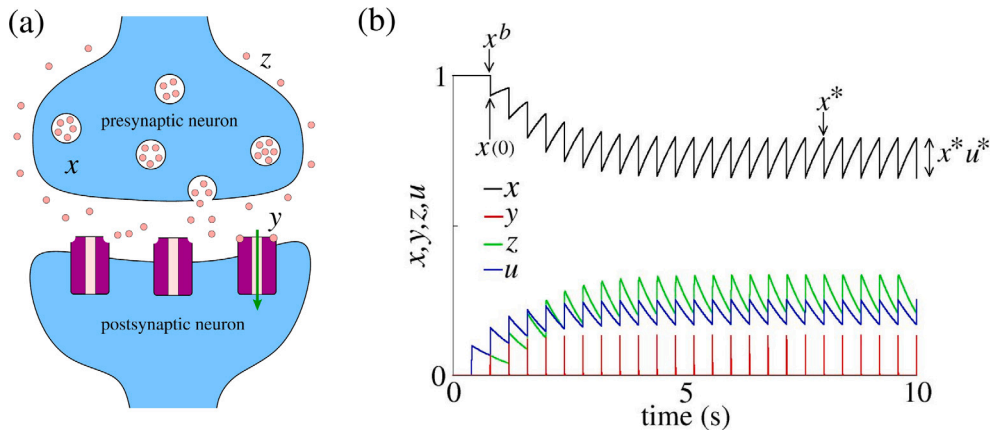
Fig. 1. (a) Schematic representation of the neurotransmitter states in a synaptic connection. x , y , and z stand for recovered, active, and inactive neurotransmitters, respectively. (b) Variable evolution x , y , z , u overtime for the facilitation regime. x^b and x(0) stand by the x variable immediately before and after the spike event, respectively. x^* stands the fixed point of x after the transient time immediately before the spike event in the periodic spike regime. x^*u^* represents the amount of neurotransmitters removed from the recovered state x and added to active state y . The same notation is used to identify the values of the variables before and after the spike event, as well as the fixed point after the transient. In Figure (b), we fixed U = 0.1 and F = 2.5 Hz.
