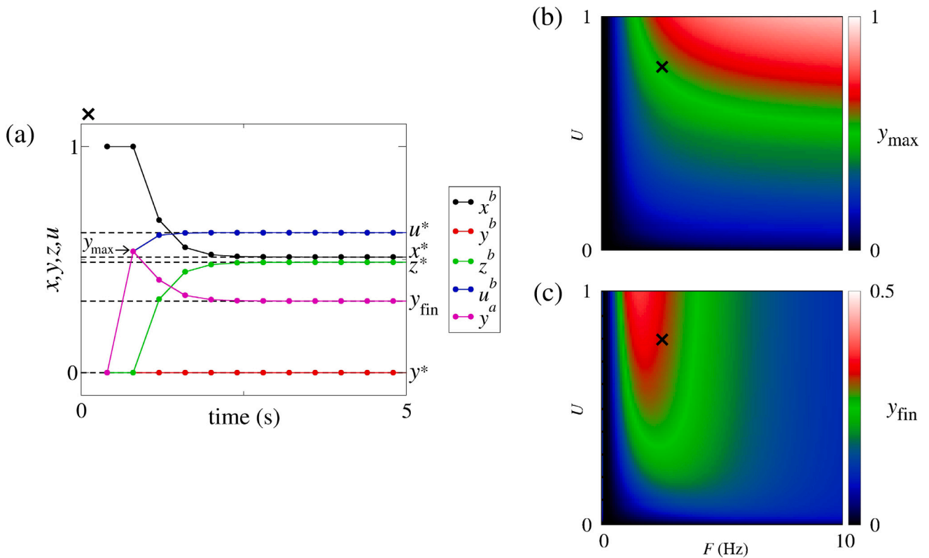
Fig. 3. (a) Time evolution of the variable values immediately before considering the spike event on the synaptic model described by the ODE ( x^b, y^b, z^b, u^b ). As the y variable is responsible for generating the current in the postsynaptic neuron, the value of y immediately after considering the spike event ( y^a ) and y_{max} , are also indicated in the figure. The black dashed lines represent the calculated equilibrium points, x^* , y^* , z^* , and u^* of the discrete map, as well as the final value y_{fin} . The parameters U = 0.8 and F = 2.5 Hz are indicated in figures (b) and (c) by a black X. (b) Maximal y values in the parameter space U \times F . y_{max} is obtained as the maximal value of y in the entire temporal evolution of the model. (c) y_{fin} in the equilibrium point, which is the y amplitude immediately after each spike past the transient time.
