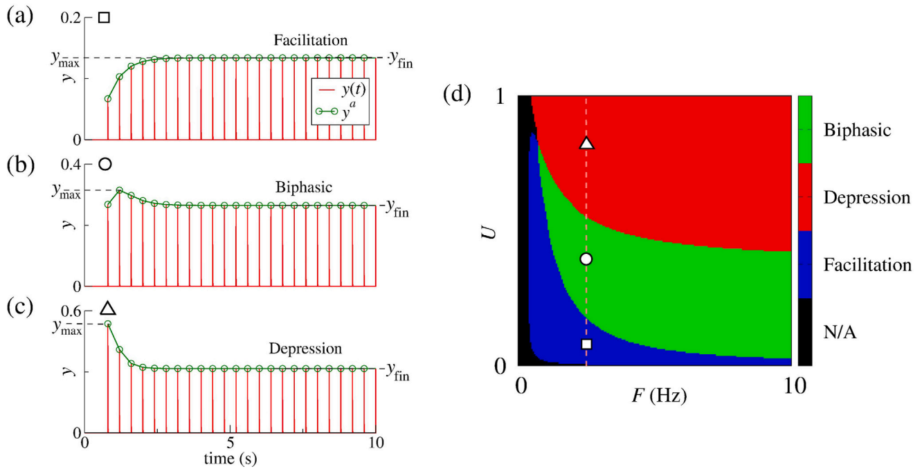
Fig. 2. (a–c) Dynamics of the active neurotransmitters in the synapse for three different regimes, (a) facilitation, (b) biphasic, and (c) depression. Red lines show the dynamics of active neurotransmitters represented by the y variable, and the green line with circles represents the y amplitude immediately after the spike event, y^a = y(0) . In Figs. (a–c), we consider F = 2.5 Hz, (a) U = 0.1 for facilitation, (b) U = 0.4 for biphasic, and (c) U = 0.8 for depression regime. In Figs. (a–c), the maximal value of y overtime is identified as y_{\max} while the final amplitude of y is represented by y_{\text{fin}} . (d) Regimes found in the dynamics synapses: facilitation, depression and biphasic. The facilitation and depression regimes are identified by means of Eqs. (45) and (46). If both conditions of Eqs. (45) and (46) are satisfied over time we identified the biphasic regime. The parameters U and F considered in Figs. (a–c) are indicated in Fig. (a). (For interpretation of the references to colour in this figure legend, the reader is referred to the web version of this article.)
