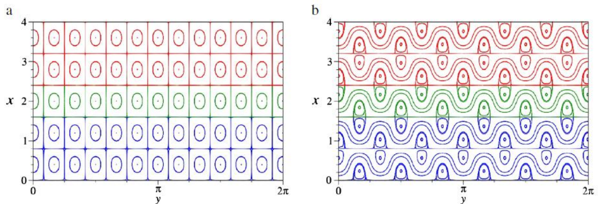
Fig. 7 Phase portrait of the dynamical system obtained from the integrable one-wave Hamiltonian (13) with a U = 0 and b U = 0.6
