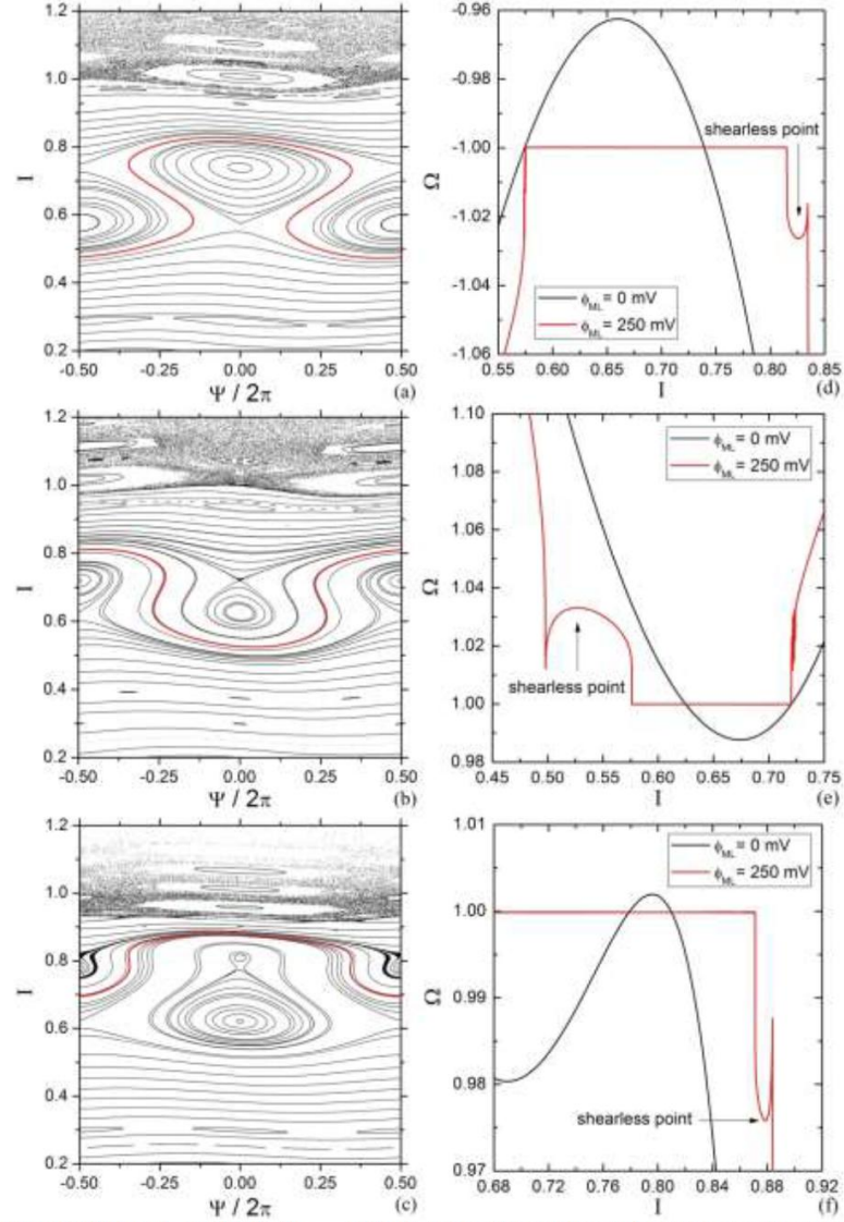
FIG. 4. Poincaré maps for potential mode amplitude \phi_{ML} = 250 mV and positive uniform velocity (a), negative uniform velocity (b) and sheared velocity (c) profiles showed in Fig. 2. The shearless curves are depicted in red in (a), (b) and (c). For these maps we used a non-monotonic safety factor profile showed in Fig. 1(b). Rotation number profiles at \Psi/2\pi = 0 for positive uniform velocity (d), negative uniform velocity (e) and sheared velocity (f).
