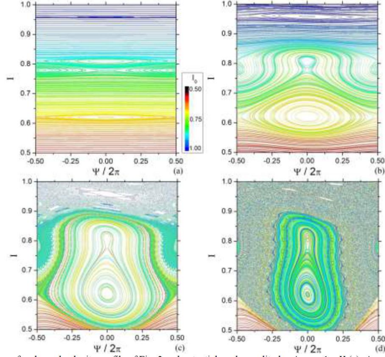
FIG. 8. Symplectic maps for sheared velocity profile of Fig. 2 and potential mode amplitudes \phi_{ML} = 1 mV (a), \phi_{ML} = 65 mV (b), \phi_{ML} = 300 mV (c) and \phi_{ML} = 500 mV (d). The color scale in these maps indicates the initial radial particle positions showed in (a).
