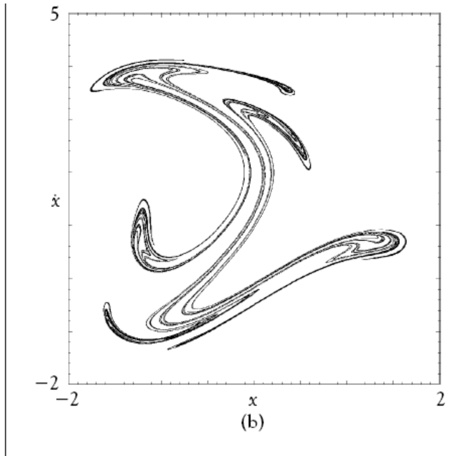
Figure 9.11 Time- 2\pi map of the forced damped double-well Duffing equation.
