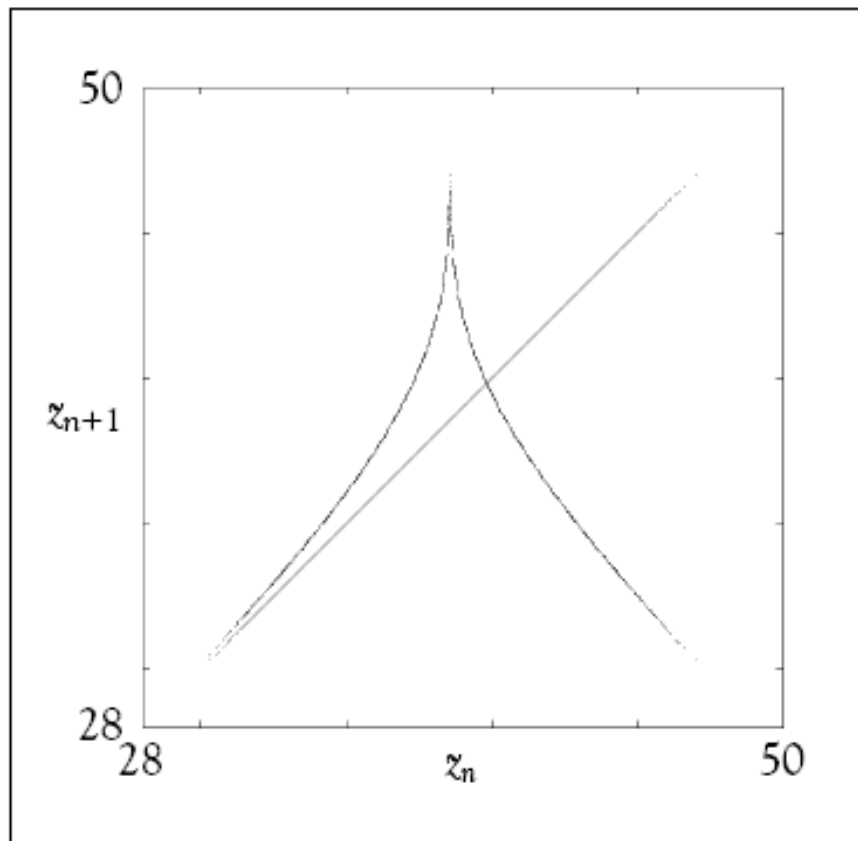
Figure 9.3 Successive maxima of z-coordinate of Lorenz attractor.
