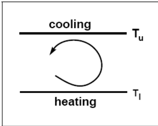
Figure 9.1 Rayleigh-Bénard convection.
