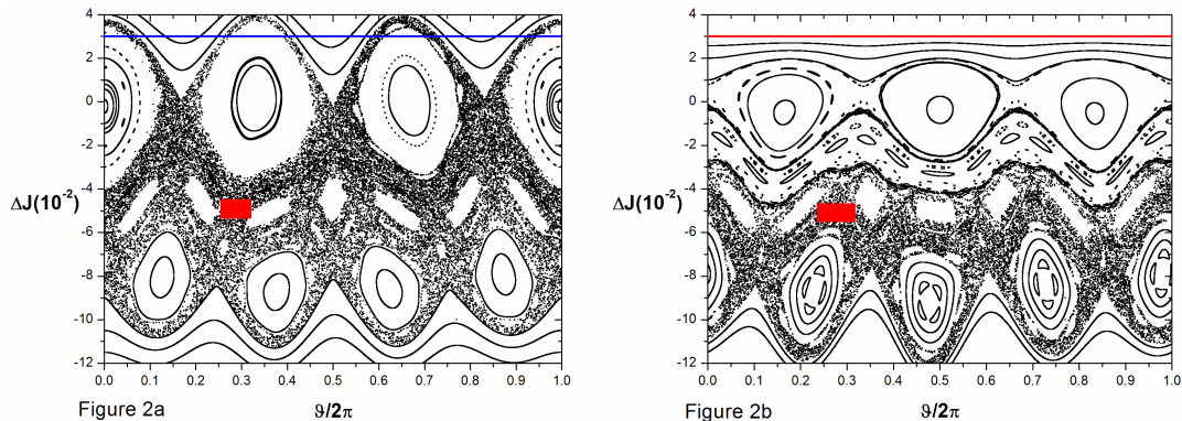
Figure.2. Poincaré sections for the resonant modes (1:3) and (1:4) with \alpha=0 for: (a) Twist map, Eq. (4), without RT with \beta = -6.0 \times 10^{-4} and \eta = 2.99 \times 10^{-4} , the blue line at \Delta J=3 is only to guide the eyes, it is not a RT. (b) Twist map, Eq.(5), with RT (in red) at \Delta J=3 , with \beta = -7.5 \times 10^{-3} and \eta = 8.2 \times 10^{-3} .
