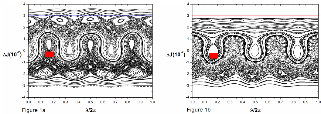
Figure.1. Poincaré sections for the resonant modes (1:3) and (1:4) for \alpha=160.15 : (a) Non-twist map, Eq. (4), without RT with \beta = -1.3 \times 10^{-4} and \eta = 1.15 \times 10^{-4} , the blue line at \Delta J=3 is only to guide the eyes, it is not a RT; (b) Non-twist map, Eq. (5), with RT (in red) at \Delta J=3 , with \beta = -4.0 \times 10^{-3} and \eta = 9.2 \times 10^{-3} .
