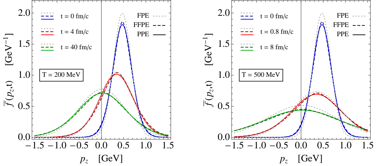
Figure 1: Plots of the distribution functions integrated out in transverse momenta, \bar{f}(p_z, t) \equiv \int_{-\infty}^{\infty} dp_x dp_y \bar{f}(\mathbf{p}, t) with \bar{f}(\mathbf{p}, t) \equiv f(\mathbf{p}, t)/\lambda^3 , as a function of p_z for several values of t , for temperatures T = 200 MeV (left) and T = 500 MeV (right). Solid and dashed lines correspond to q = 1.10 , and dotted lines to q = 1 . We have considered the rest mass of the heavy quark m_0 = 1.5 GeV, its initial momentum p_o = 0.47 GeV in the z -direction corresponding to the initial speed v_o = 0.30 c , the initial width \sigma_o = 0.2 GeV, while (A = 0.0820 \text{ fm}^{-1}, B = 0.0216 \text{ GeV}^2/\text{fm}) for T = 200 MeV (left panel) and (A = 0.381 \text{ fm}^{-1}, B = 0.228 \text{ GeV}^2/\text{fm}) for T = 500 MeV (right panel). We have considered \lambda = 1 GeV for the multiplicative factor of the distribution function.
